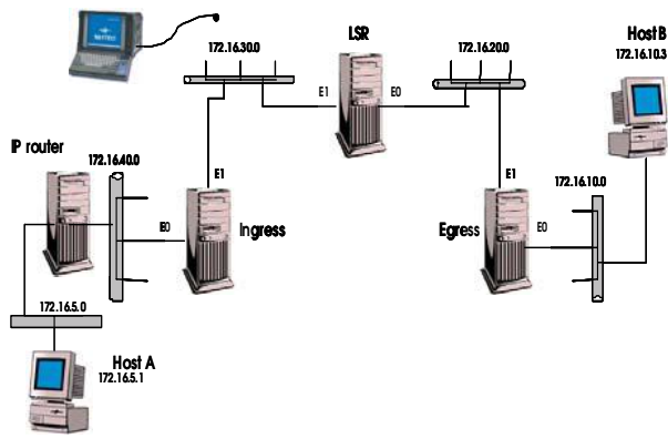
Fig. 1. Test-bed's architecture
